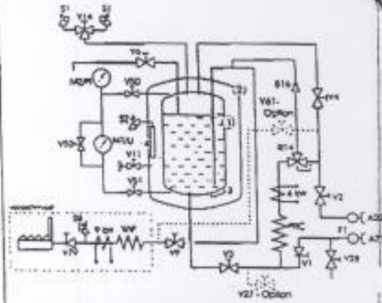
Figure 7.4.2 Flow diagram for a carbon dioxide tank
